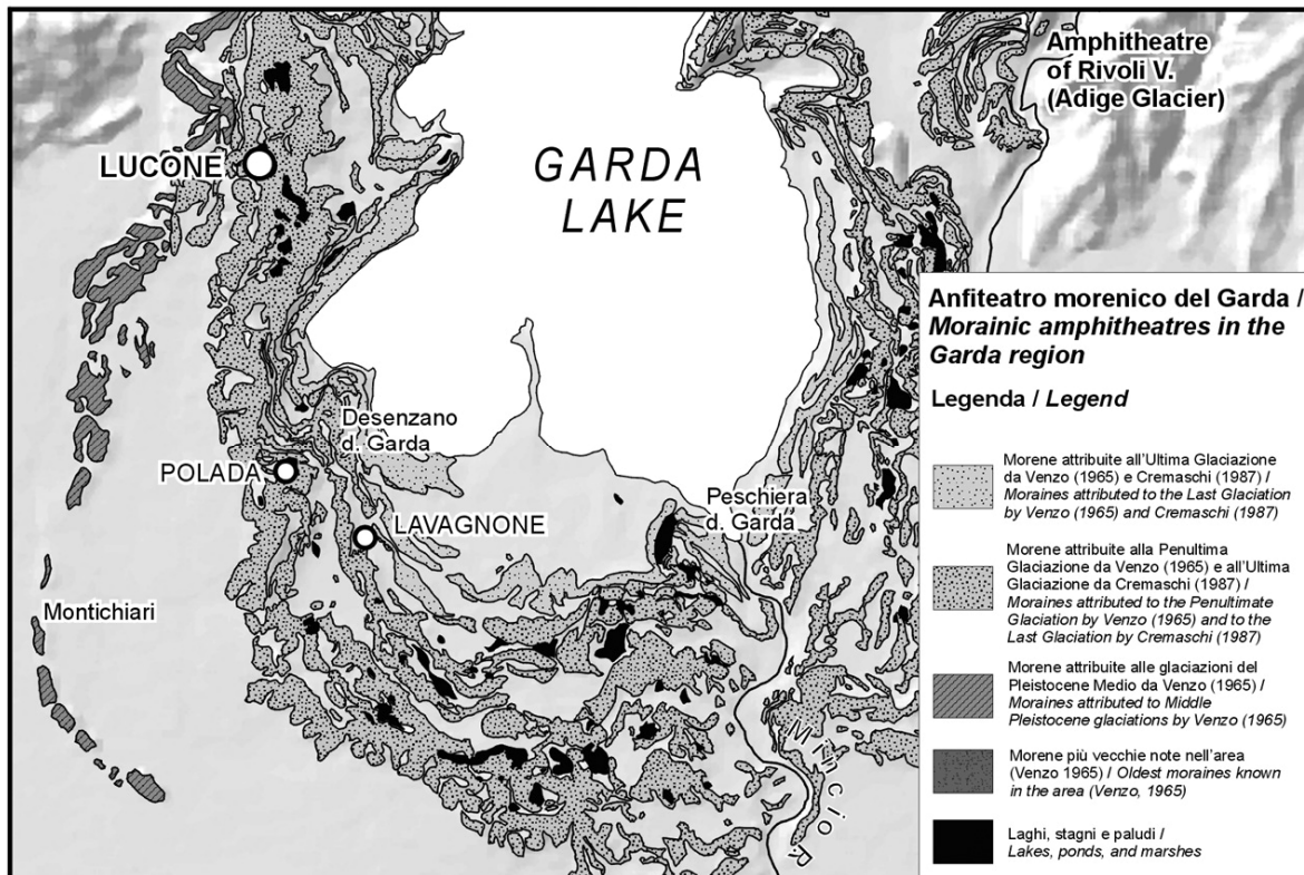
Fig. 1, The Lucone basin (Polpenazze del Garda, Brescia) is located in the western part of the morainic amphitheatre of Garda Lake.
