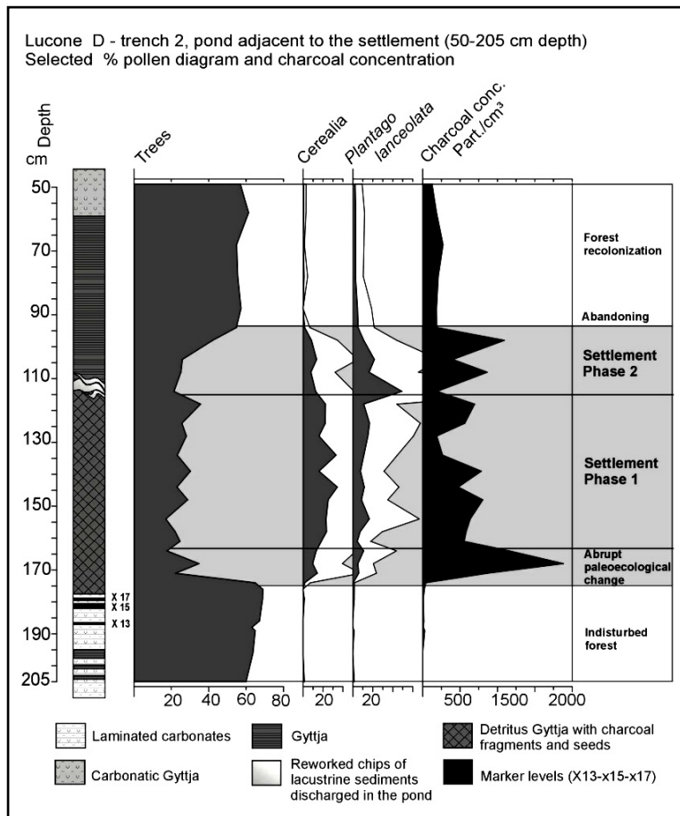
Fig. 2, Summary pollen curves and general evolution of "Lucone D" pile-dwelling. The settlement foundation is marked by a fire and correlated to a sudden reduction in forest cover and cereals % pollen curve expansion.
