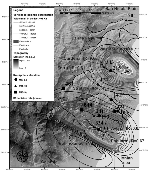
Fig. 1 - Knickpoints elevation and incision rates compared with the deformation model.
