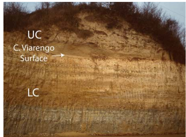
Fig. 9 - Alternating planar bedded silt and cross-bedded fine sand of the San Martino Unit (LC), separated by the coarse, cross-bedded sand of the C. Gherba Unit (UC) by the Cascina Viarengo erosional Surface. The newly exposed sediments (at the base of the outcrop) preserve the typical grey colour of the San Martino Unit, not involved in the surficial weathering that involves the exposed for longer sediments, whose yellowish color is due to the lengthy subaerial exposure. Cascina San Martino Quarry in Villafranca d'Asti (central type-area).
