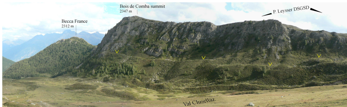
Fig. 12 - In the northern slope of the Becca France ridge, a uphill-facing scarp (arrows) develops, linked to the DSGSD phenomenon.
