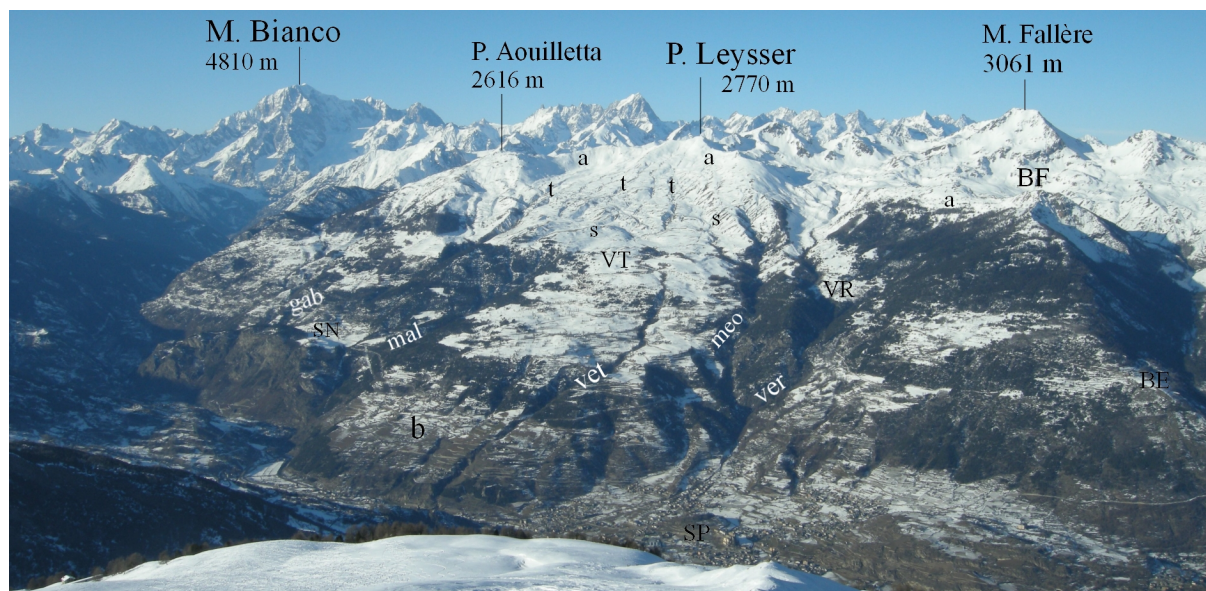
Fig. 8 - The P. Leysser DSGSD shows a remarkable main scarp, arched in plan, just below the crest (a). Its a distal sector (b), expanded in the Aosta Valley floor, is incised by several watercourses: T. Gaboé (gab), T. Mallaley (mal), T. de Vetan (vet), T. de Meod (meo) and T. de Verrogne (ver). The gravitational landforms, as minor scarp (s) and longitudinal trenches (t), are underlain by the snow. The location of Becca France (BF) and of the villages of Vetan (VT), Verrogne (VR), Saint Nicolas (SN), Saint Pierre (SP) and Bellon (BE) are also indicated.
