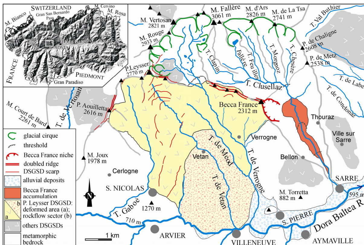
Fig. 1 - Geographical and geomorphological sketch of the area, comprising the P. Leysser DSGSD. The Becca France ridge is involved in a remarkable set of WNW-ESE doubled ridges. The Digital Terrain Model of the Aosta Valley, in which the present glaciers are mapped, shows the location of the area of investigation.
