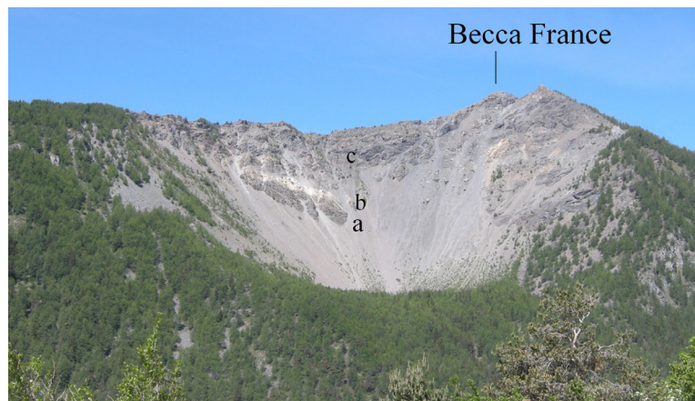
Fig. 4 - The detachment niche of the Becca France historical landslide. The tectonic contact between the Lower Calcschist Complex (a) (Lower TMU in Fig. 6) and the Upper Calcschist Complex (c) (Upper TMU in Fig. 6) is underlined by a cargneule and gypsum level (b). The niche cuts the noticeable doubled ridge developed near the summit.
