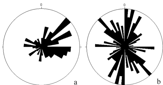
Fig. 5 - Equiareal projection (lower hemisphere) of fractures in the Becca France ridge (151 data). Dip direction (a); strike direction (b).
