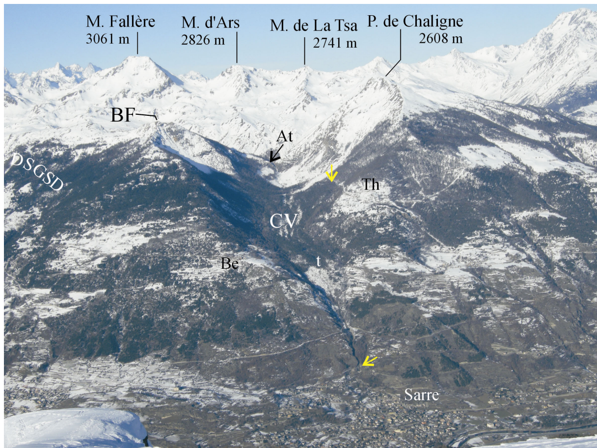
Fig. 2 - The Becca France ( BF ) historical landslide involves the Clusellaz Valley ( CV ). It shows the typical features of a tributary glacial valley, separated from the main valley by a hanging threshold ( t ). Another threshold near Arpy ( At ) divides the lower Clusellaz Valley from the upper one. A wide fluvial fan develops at the valley outlet, built from the Sarre Village. The arrows indicate the distal edge of the landslide. The location of the Bellon ( Be ) and of the present Thouraz ( Th ) villages is also indicated.
