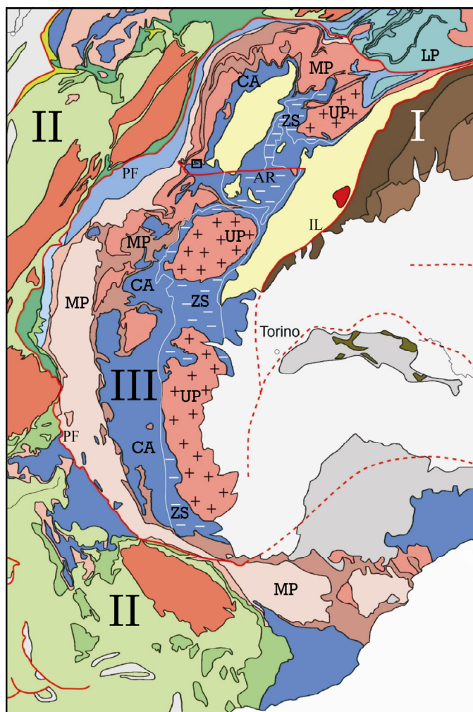
Fig. 3 - Geological schematic map of the Western Alps: (I) the internal domain, corresponding to the Southern Alps; (II) the external domain, consisting of the Helvetic-Dauphinoise domain; (III) the axial sector of the Austroalpine and Penninic continental domains, separated by oceanic units of the Piedmont Zone. IL: Insubric Line; PF: Penninic Front; AR: Aosta-Ranzola Fault; LP: Lower Penninic; MP: Middle Penninic; UP: Upper Penninic; ZS: Zermatt-Saas like-Units; CA: Combin-Aouilletta like-Units.
