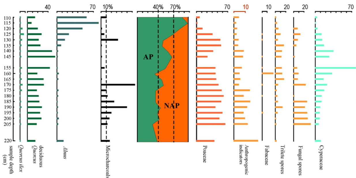
Fig. 1- Synthetic pollen diagram of Passo Murato core
