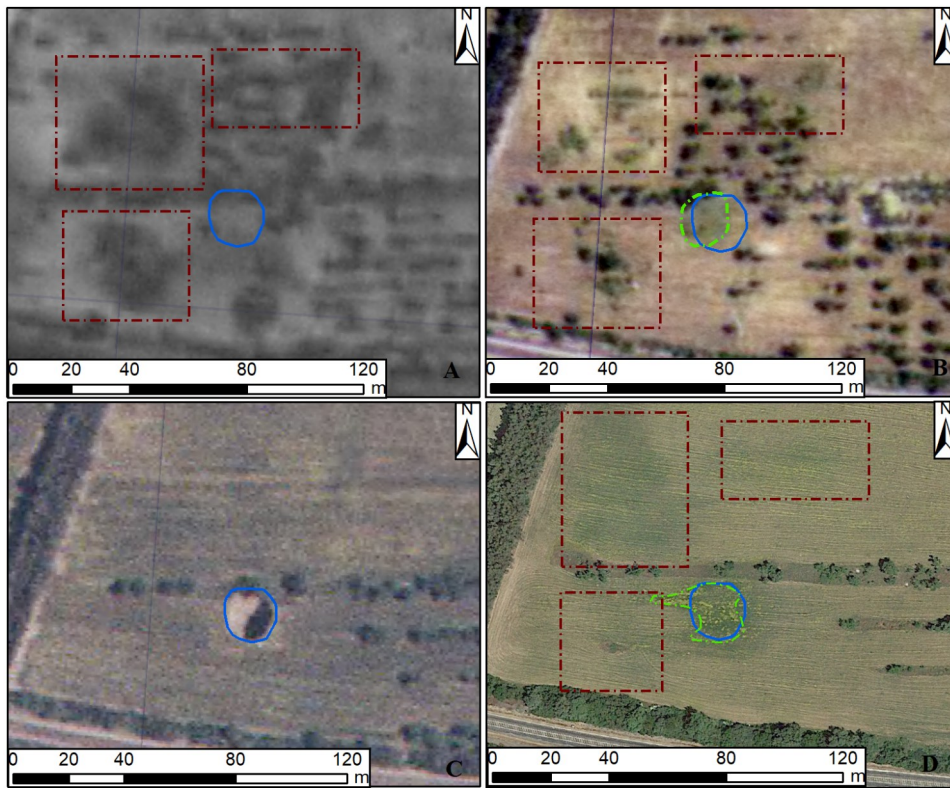
Fig. 5 - Ortophotos of the Guarda su Merti area dating 1954 (A), 1978 (B), 2010 (C), 2022 (D). Sinkhole limits in blue. In green, areas with pronounced plant growth/ herbaceous patches within and around the sinkhole. In brown rectangles areas outside the sinkhole showing dark colouring/pronounced plant growth.
