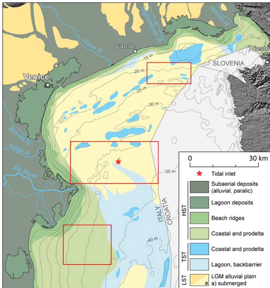
Fig. 1 - Geological map of the northern Adriatic area. The red rectangles indicate the areas where the tidal inlets are mainly concentrated. The red star indicates the position of the inlet reconstructed in Fig. 2.
