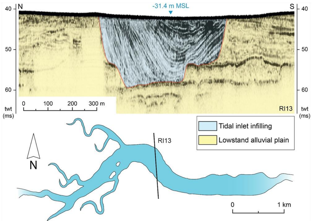
Fig. 2 - Upper portion: example of tidal inlet cross section visible in a CHIRP profile. Lower portion: reconstruction of the planform of the tidal inlet. The black line indicates the position of the CHIRP profile. After Ronchi et al. (submitted).
