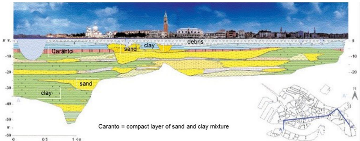
Fig. 2 - Subsoil geological setting of Venezia along a cross-section (after Zezza 2008).
