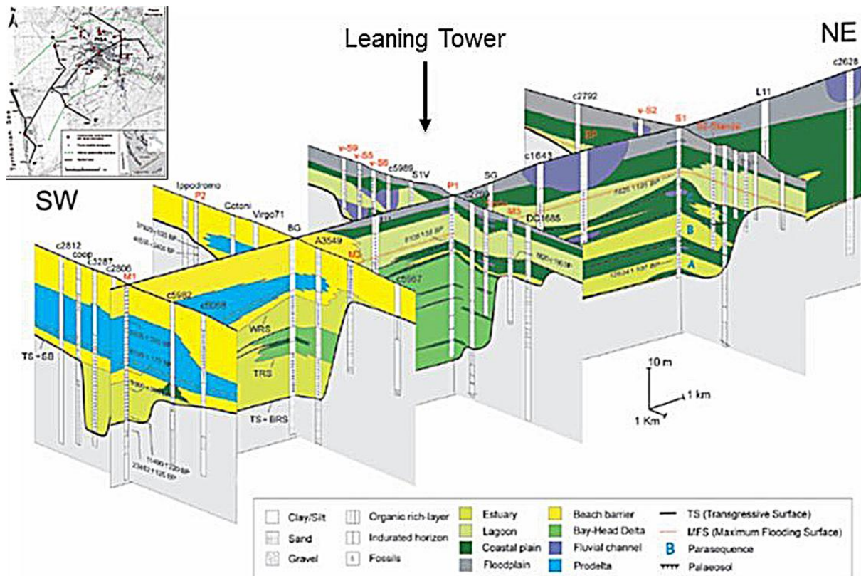
Fig. 3 - Subsoil setting of the Pisa area evidencing Arno paleo-valley during the last "Ice-Age" (after Amorosi et al. 2008).
