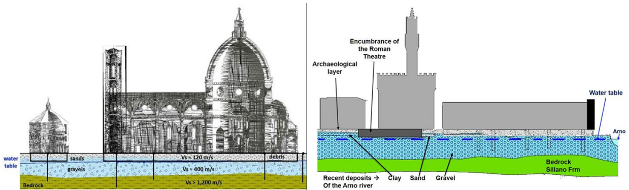
Fig. 1 - Schematic subsoil setting of the main historical buildings at Firenze.
